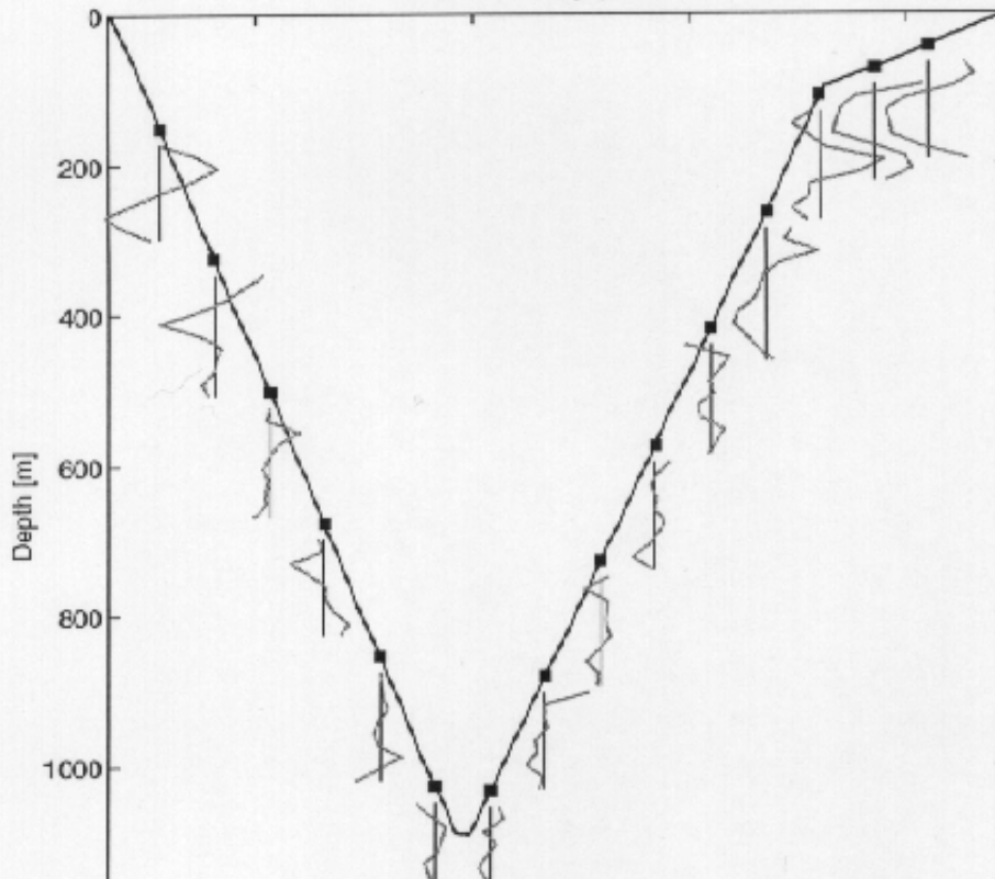
Raw velocity profiles
