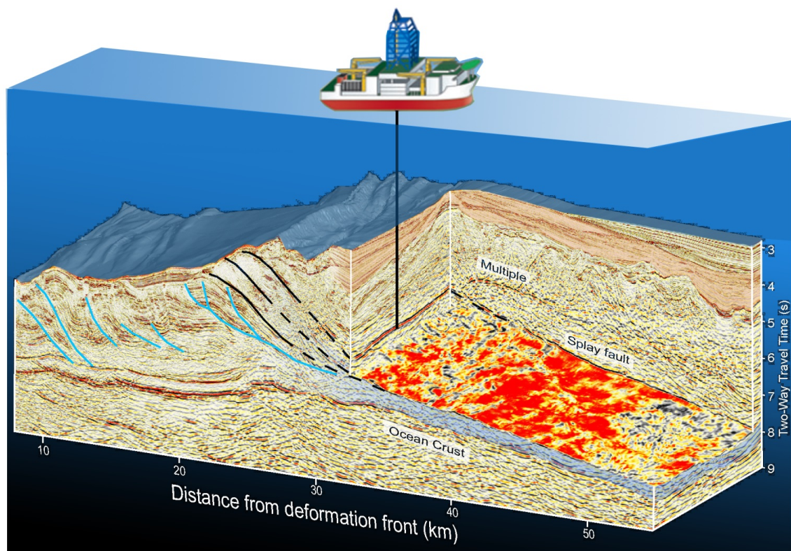
Figure A. A 3D seismic image of the Nankai Trough accretionary prism along the southwestern Japan margin, a plate boundary which has been a focus of multiple scientific ocean drilling efforts for decades. The cut-out area looks into the plate-boundary megathrust, where it intersects a major splay-fault system, shown with dipping black lines. Blue lines show thrust faults within the upper
