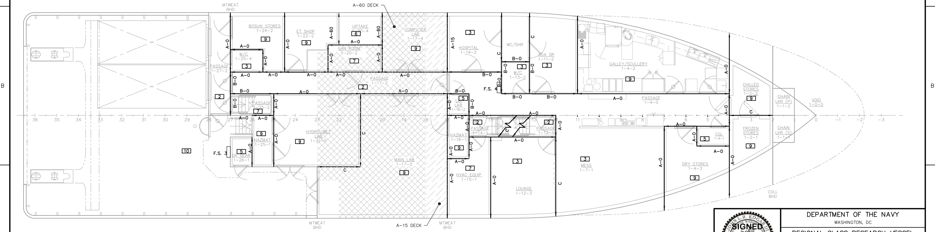
MAIN DECK PLAN 3/16"=1'-0"
