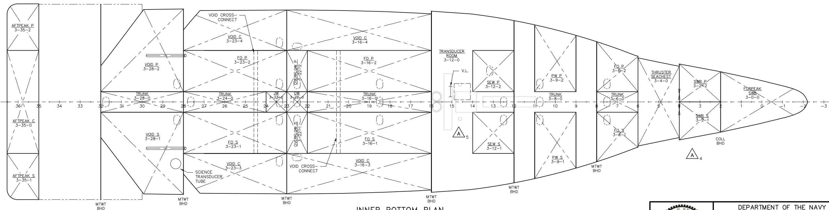
INNER BOTTOM PLAN
