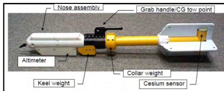
Magnetometer
