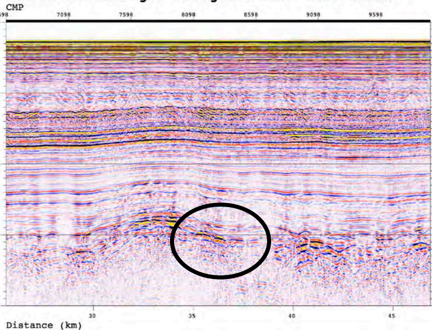
MGL1506.5 P190 Navigated Full Fold Stack
