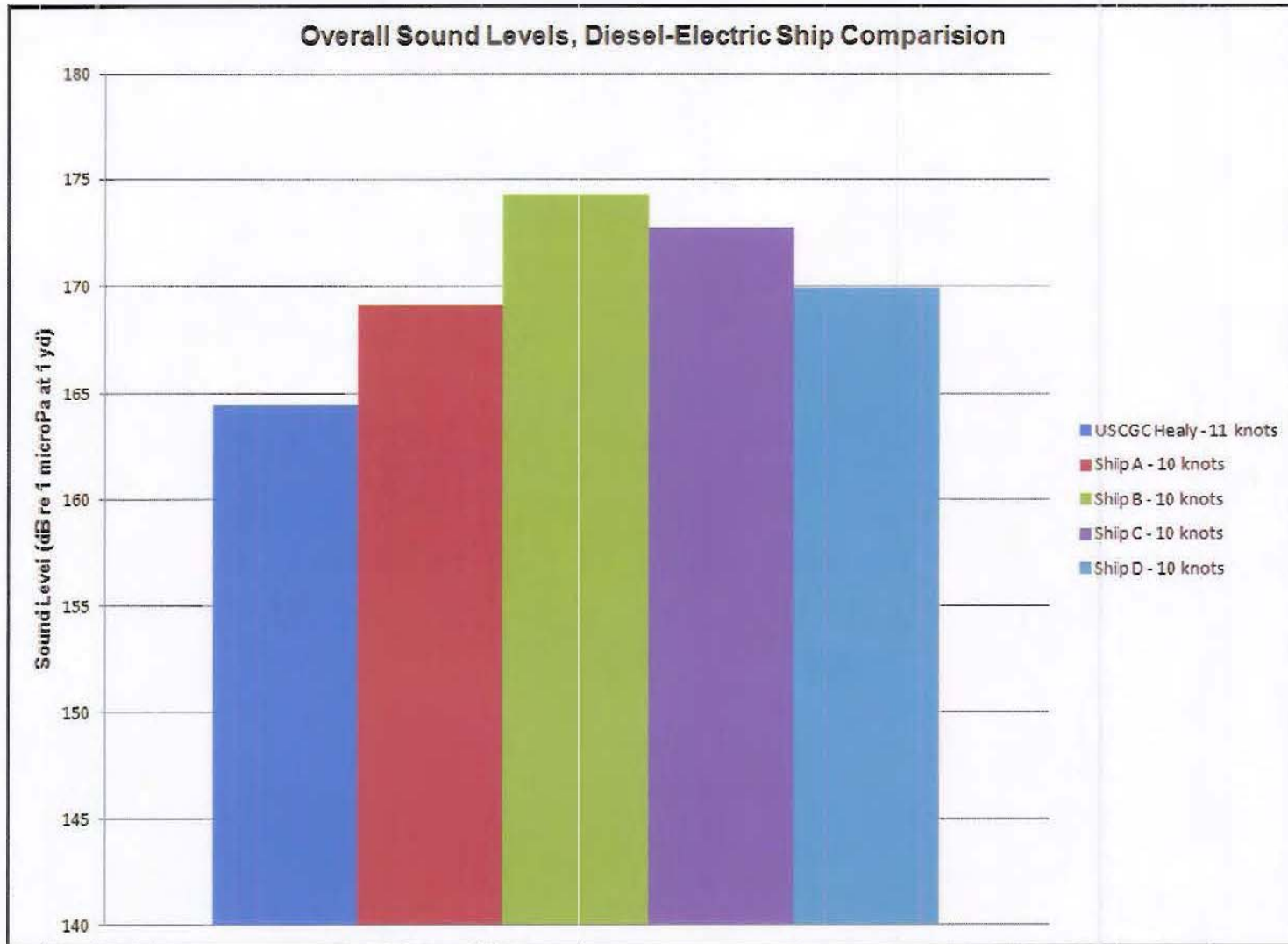
Figure 4. Healy Overall Sound Level Compared to Similar Diesel-Electric Ships
