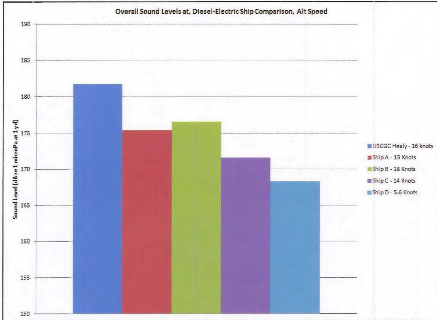
Figure 5. Healy Overall Sound Level Compared to Similar Diesel-Electric Ships, Alternate Speed
