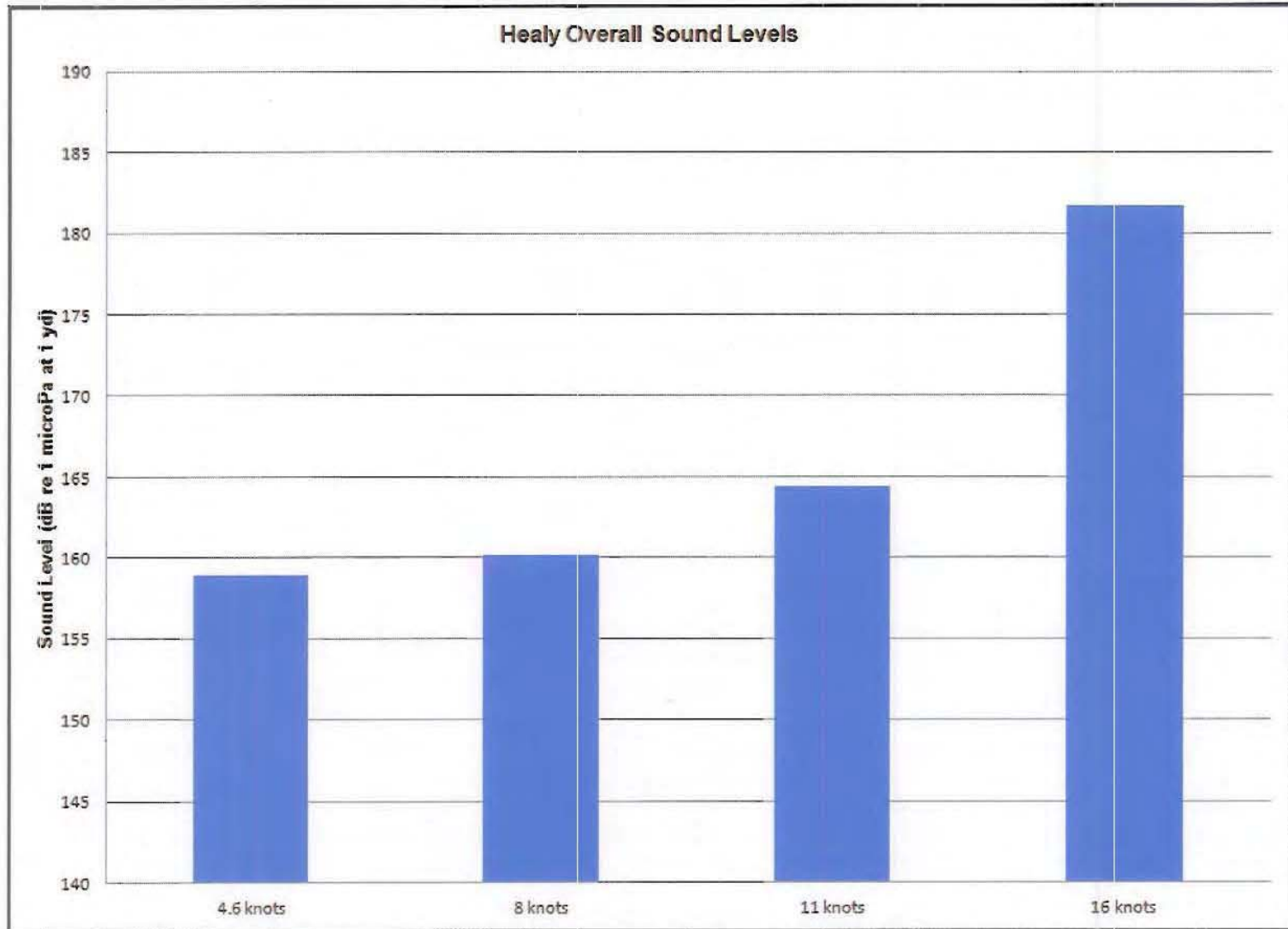
Figure 3. Healy Overall Sound Levels by Speed
