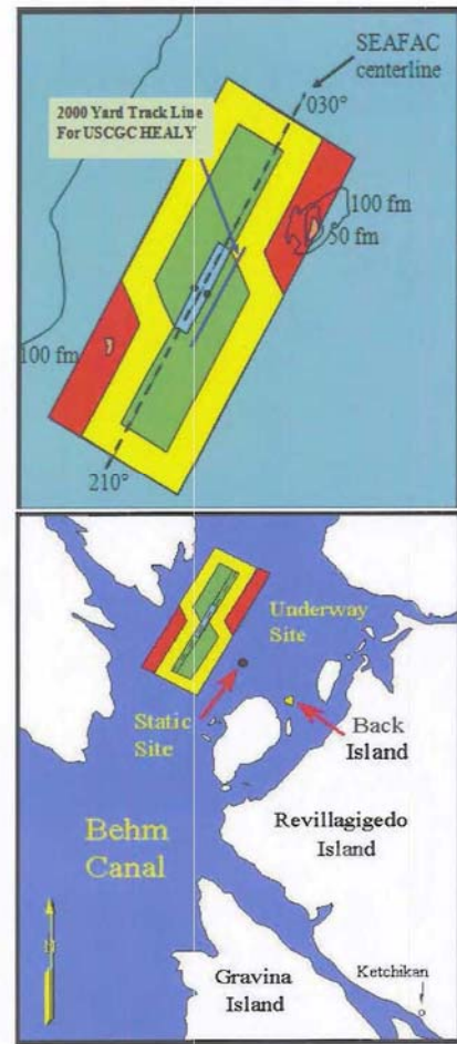
Figure 1. Southeast Alaska Acoustic Measurement Facility
