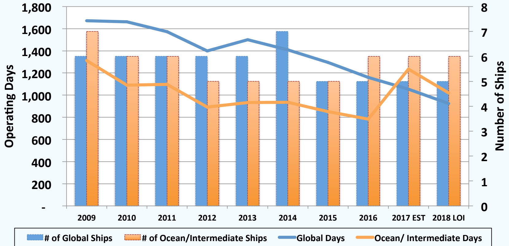
Figure 2: Ship Utilization by Class: 2009 – 2018 Global and Ocean Intermediate Classes
