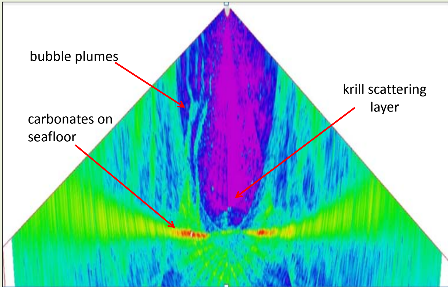
Figure Left: Unprocessed, real-time EM302 image from shipboard read-out during 2010 test cruise on THOMPSON on the Washington margin, showing methane gas plumes, zooplankton scattering layer and hard acoustic returns from pockmark carbonate plates on seafloor.
