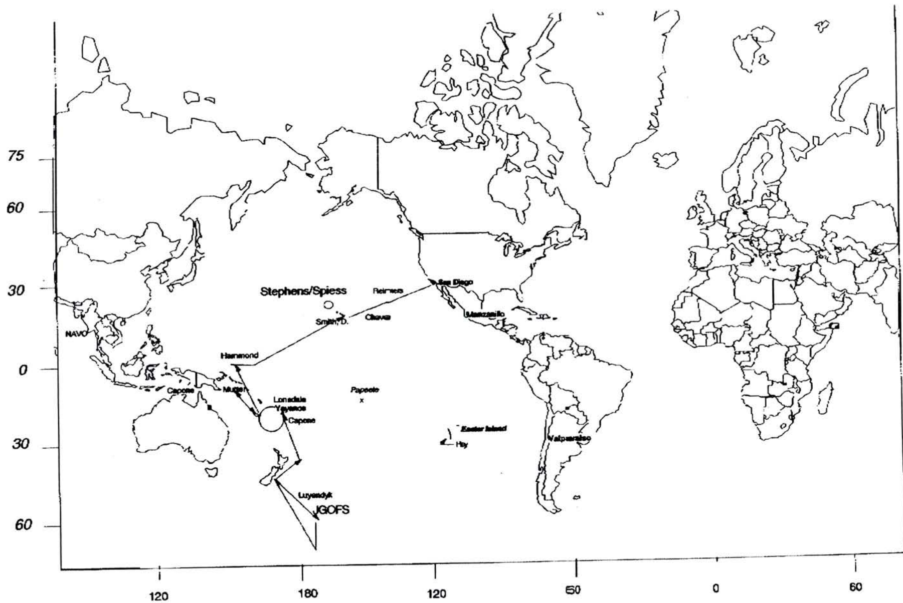
R/V Roger Revelle 98 Scripps Institution of Oceanography
