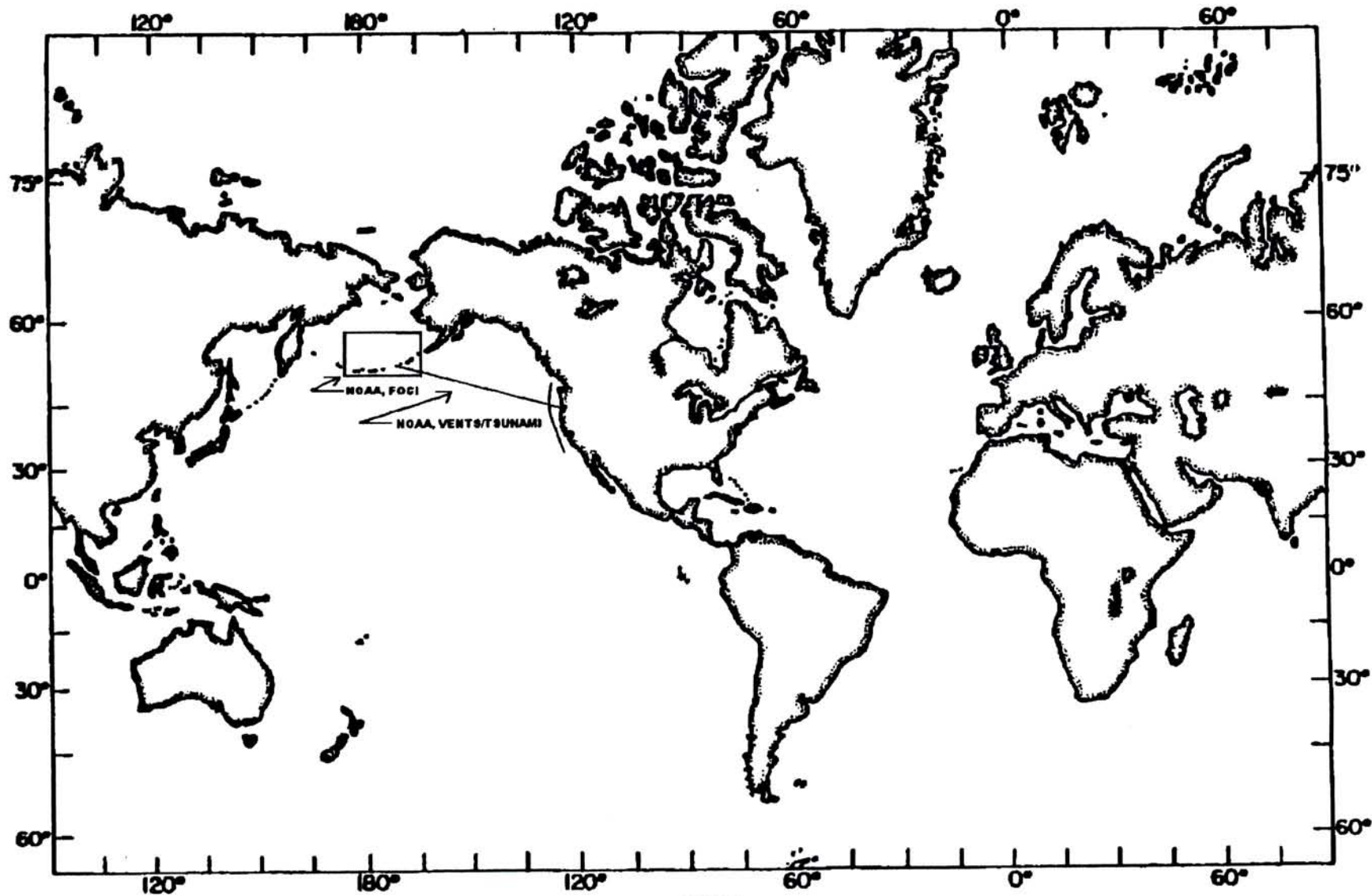
1998 CRUISE TRACKS R/V WECOMA OREGON STATE UNIVERSITY
