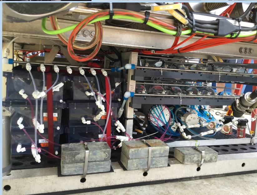
Hydrothermal Organic Geochemistry Sampler (HOG Sampler)
