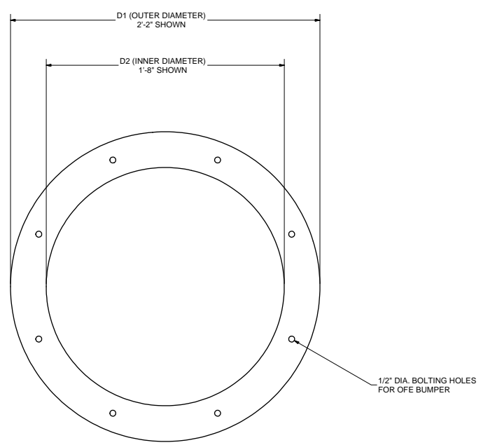
DETAIL B LOWER DOCKING RING PLAN VIEW - SCALE: 6"=1'-0"
