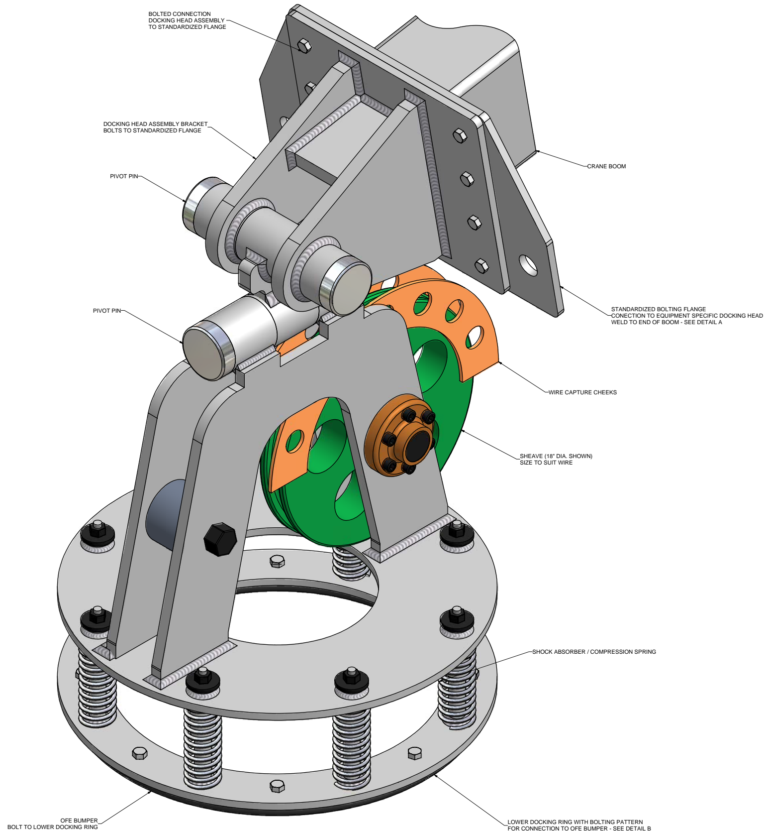
DOCKING HEAD ASSEMBLY ISOMETRIC VIEW - SCALE: 6"=1'-0"
