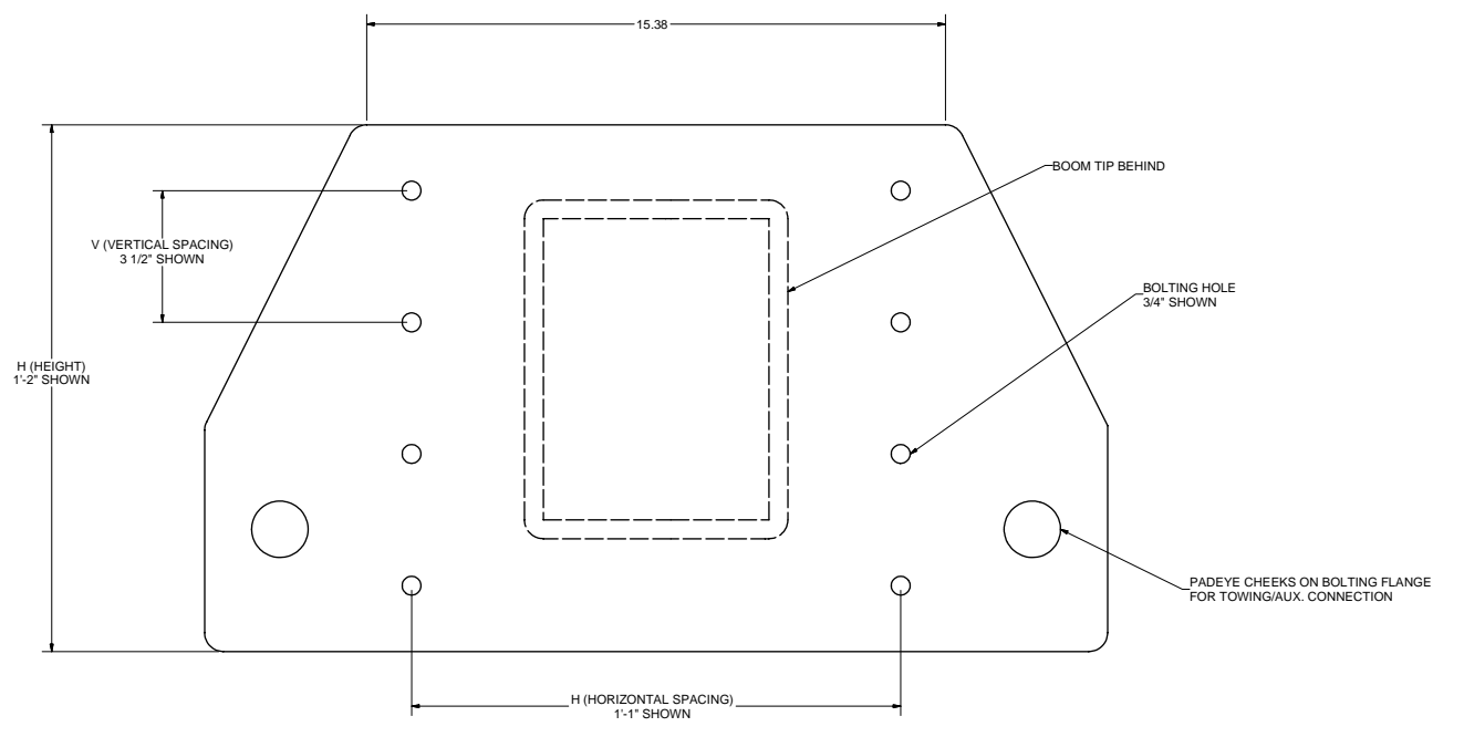
DETAIL A STANDARDIZED BOLTING FLANGE PLAN VIEW - SCALE: 6"=1'-0"
